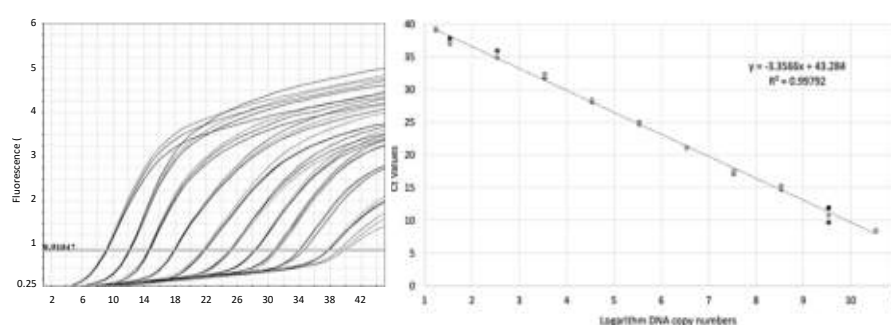
Figure 2. (a) Amplification plots by GRLDaV real-time qPCR for three replicates of serial dilutions of plasmid DNA containing the GRLDaV target region. (b) Quantitation standard curve generated. Both the mathematical equation of the curve and the coefficient of correlation ( R^2 ) are indicated.
