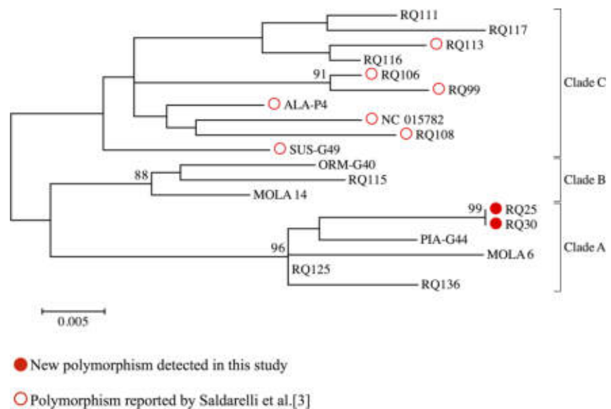
Fig 4. Phylogenetic analysis of Spanish GPGV isolates by Maximum likelihood method. Trees were generated under the Tamura 3 model of nucleotide substitution. Branches supported by a minimum of 75% of 2,000 bootstrap replicates.
