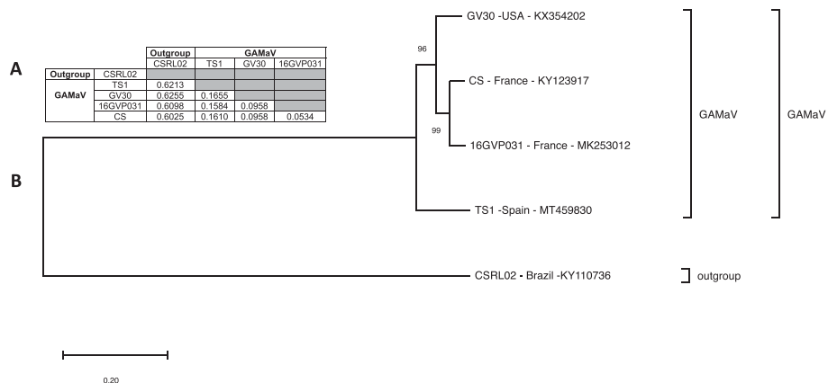
Figure S1. A. Estimates of evolutionary divergence between sequences. The number of base substitutions per site between sequences are shown. Analyses were conducted using the Tamura-Nei model. B. Phylogenetic tree constructed with available full-length GAMaV isolates inferred by Maximum Likelihood method and Tamura-Nei model by MEGA X. The isolates are identified by their accession numbers and origin. The scale bar shows a genetic distance of 0.20. Bootstrap percentages (500 re-samplings) are indicated on the branches. Sequence of citrus sudden death-associated virus (KY110736) isolate is used as outgroup reference.
