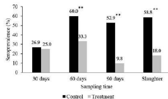
Figure 1. Salmonella seroprevalence (cut-off value OD% \geq 40 %; Herdcheck Swine Salmonella ELISA test, IDEXX Laboratories, US) at different sampling times in the fattening period in the control and treatment group. **: p < 0.01
