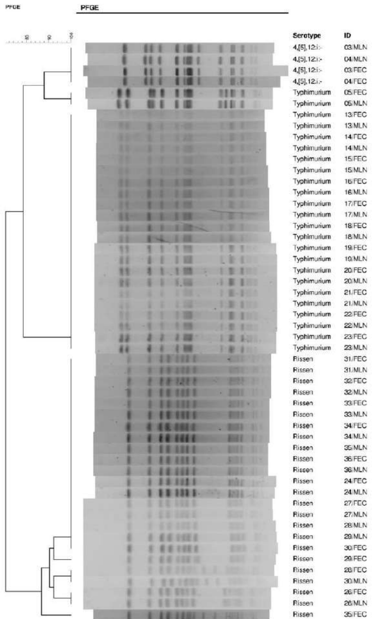
Fig. 4. Dendrogram showing the genetic relatedness between Salmonella isolates from faecal (FEC) and mesenteric lymph nodes (MLN) samples from infected pigs from group C.
